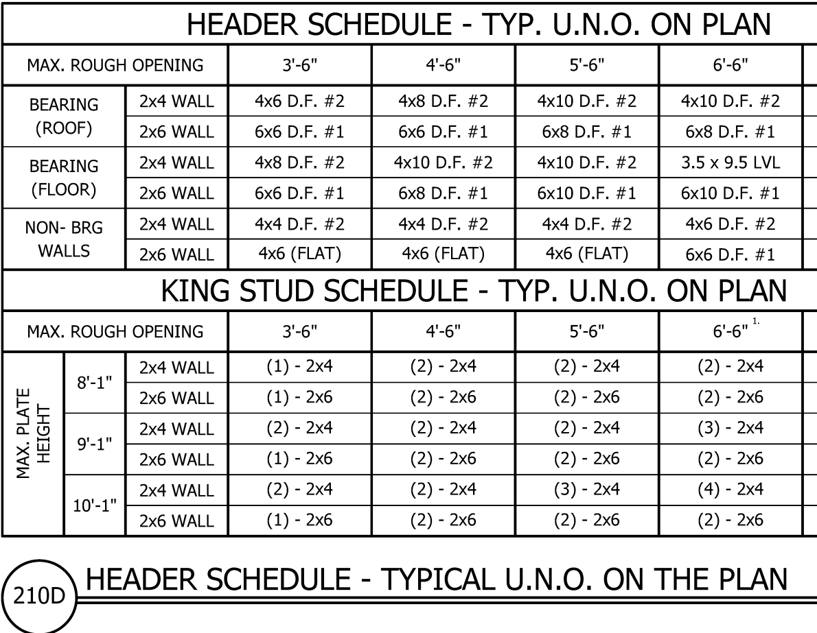
210C HEADER AT CORNER POST - ELEVATION and 210D HEADER SCHEDULE - TYPICAL U.N.O. ON THE PLAN
