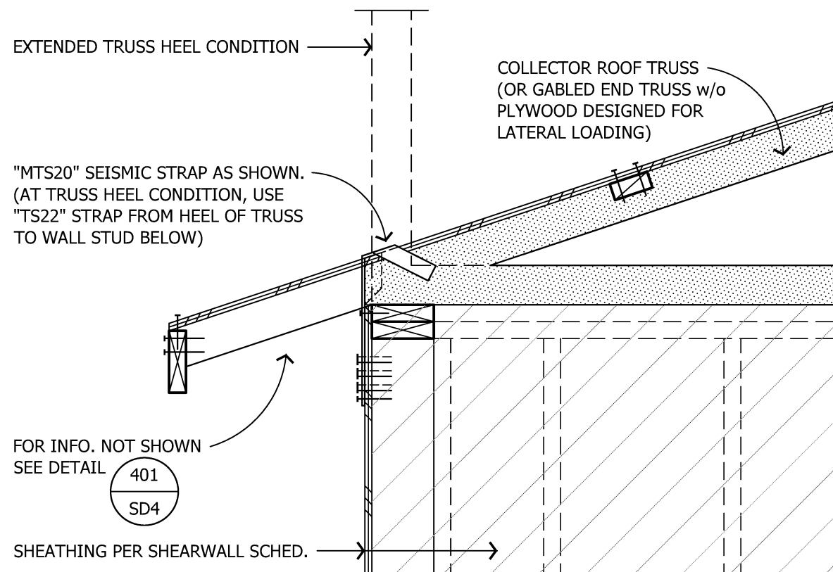
406 COLLECTOR TRUSS UPLIFT ANCHORAGE
