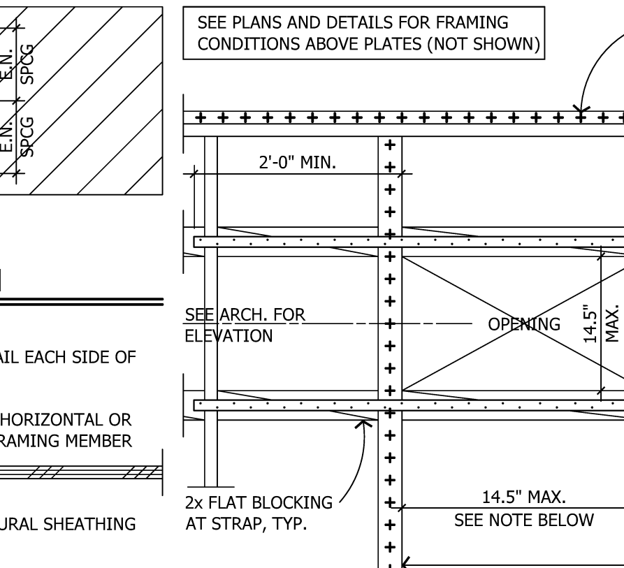
105B ELEVATION
