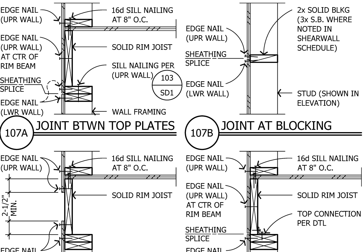
107A JOINT BTWN TOP PLATES
