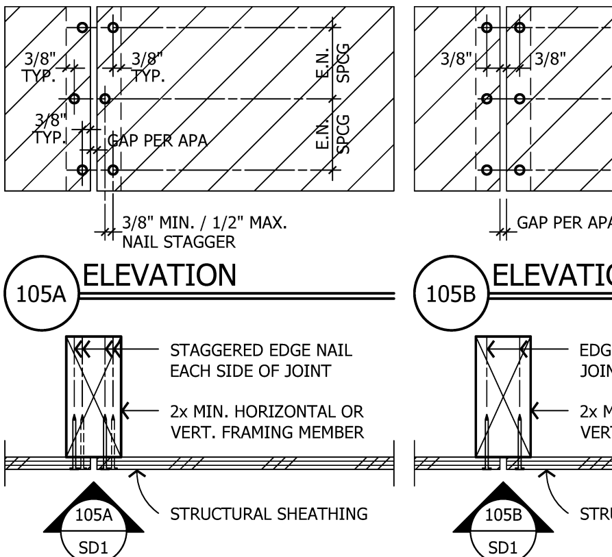
105A ELEVATION
