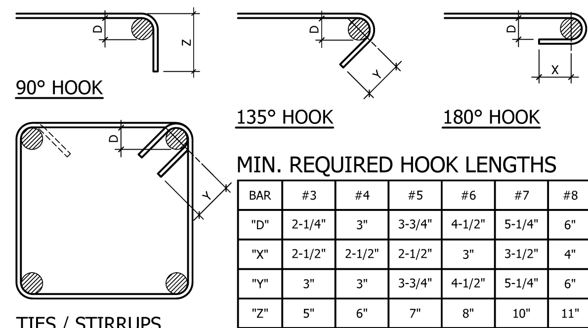
203 STD REINF. HOOKS - DOUBLE ROW
