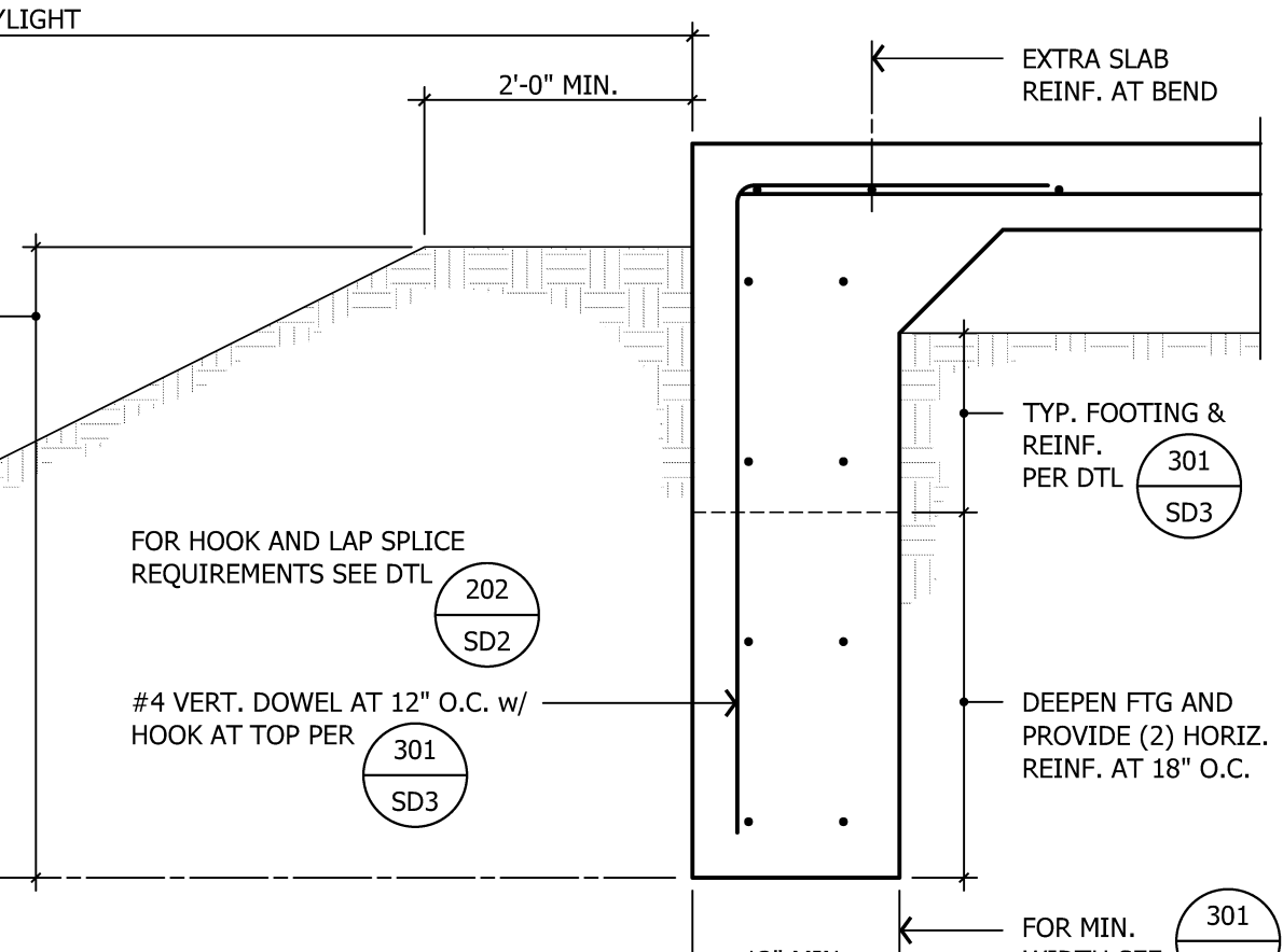
209 TOP PLATE SPLICES, BREAKS AND PENETRATIONS
