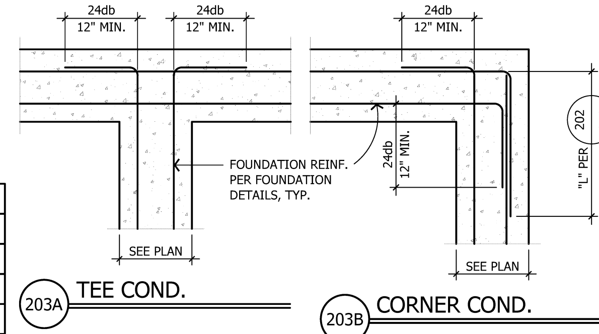
203A TEE COND. and 203B CORNER COND.
