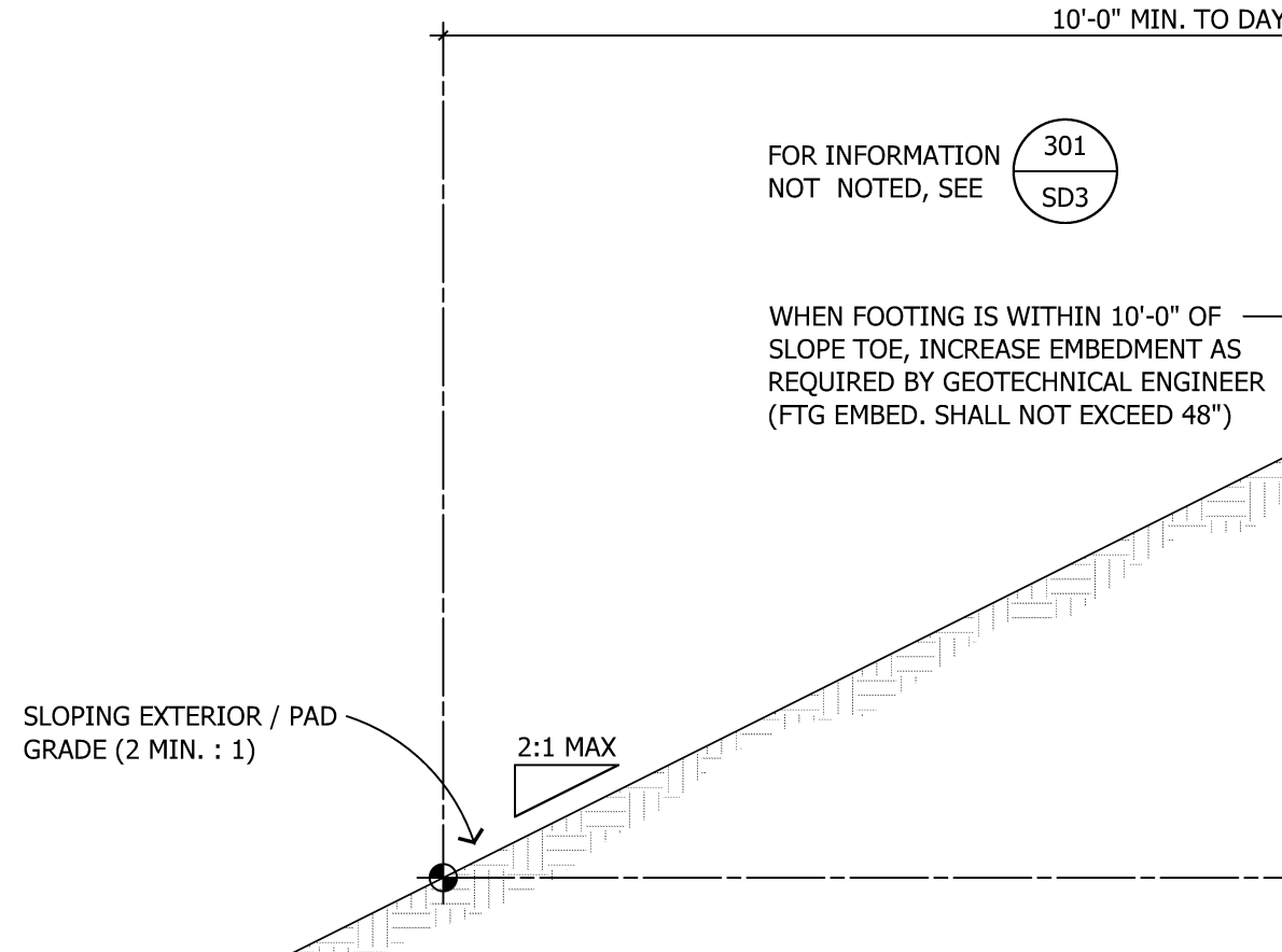
208 INCREASED FOOTING DEPTH BY SLOPE
