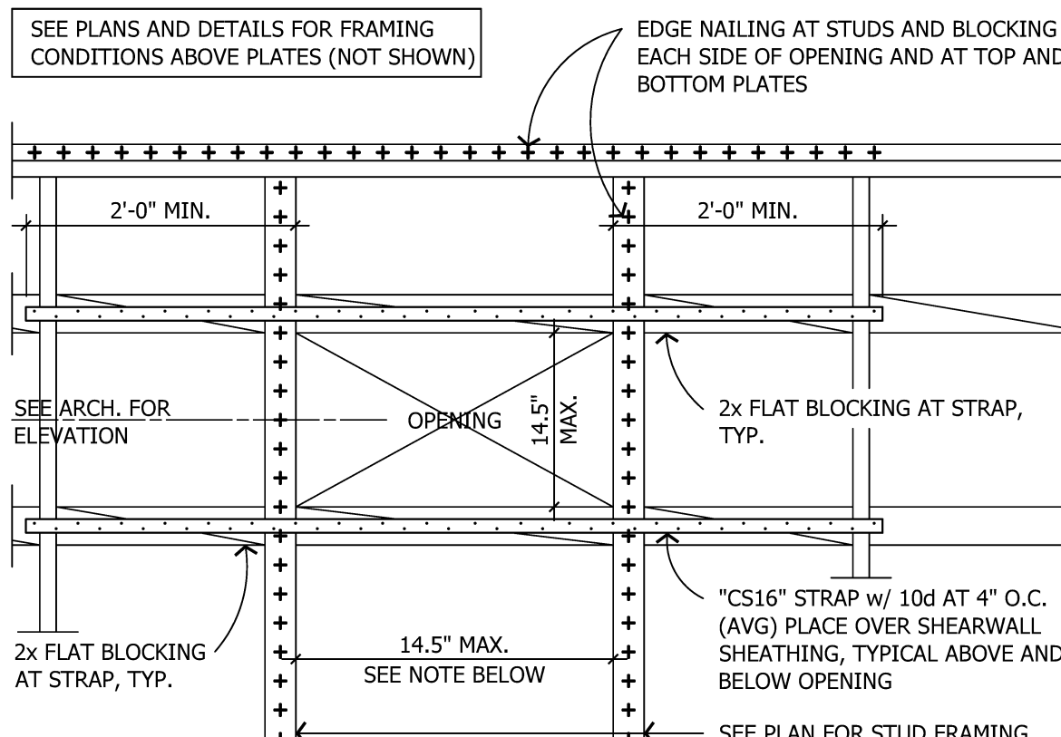
105B ELEVATION
