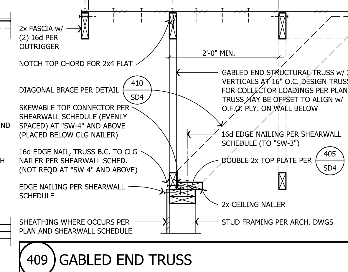
409 GABLED END TRUSS
