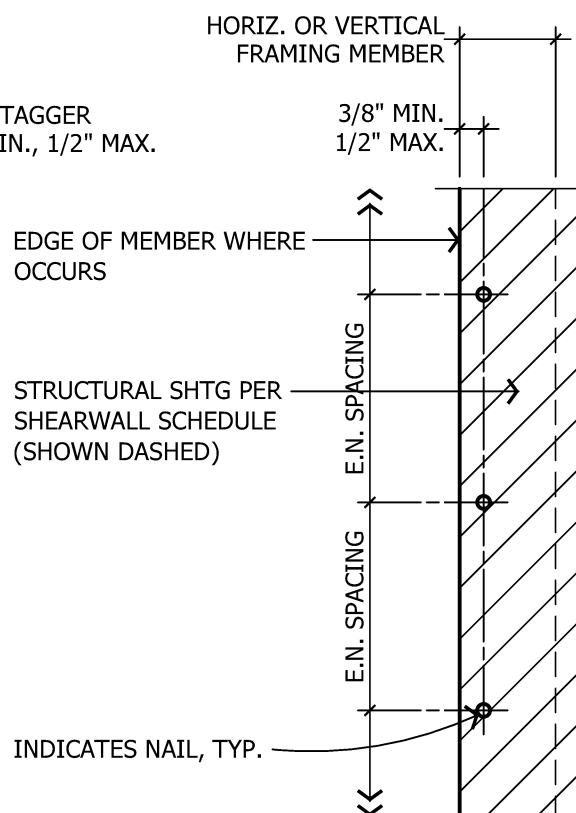
104B STANDARD NAILING AT SPACE OF 4" OR GREATER
