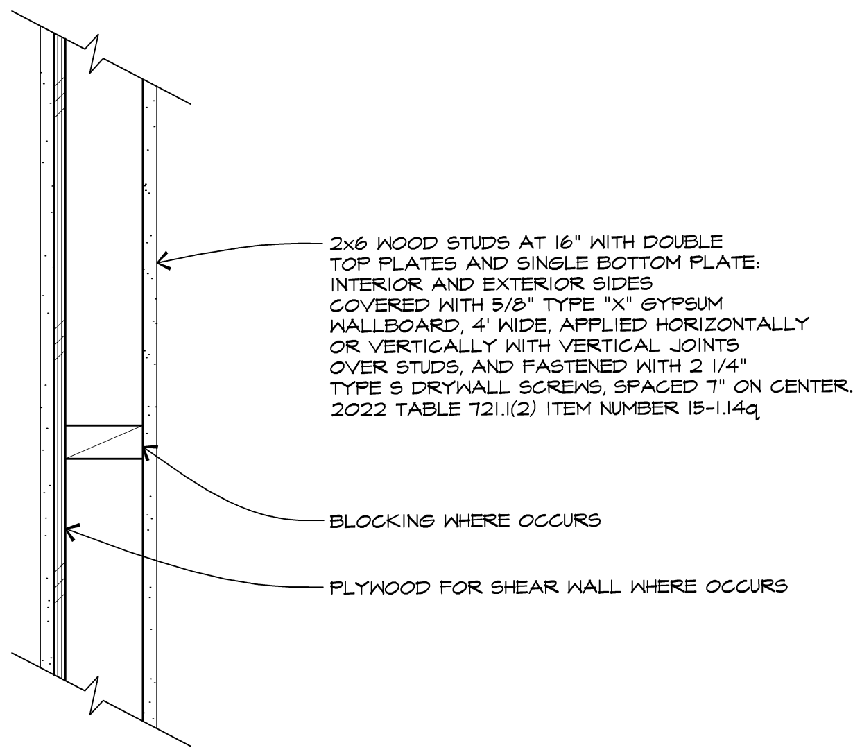
1 HOUR FIRE RATED WALL DETAIL
