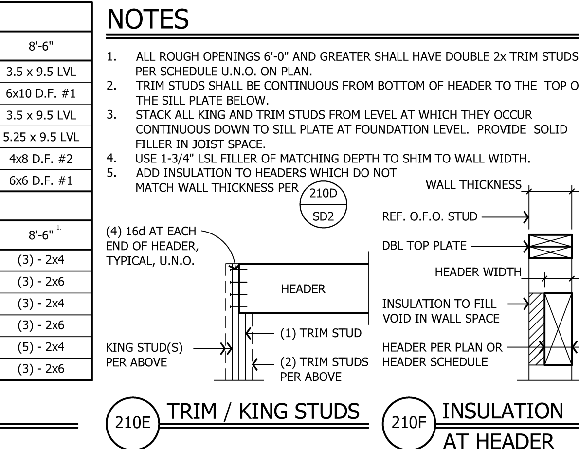
210E TRIM / KING STUDS and 210F INSULATION AT HEADER
