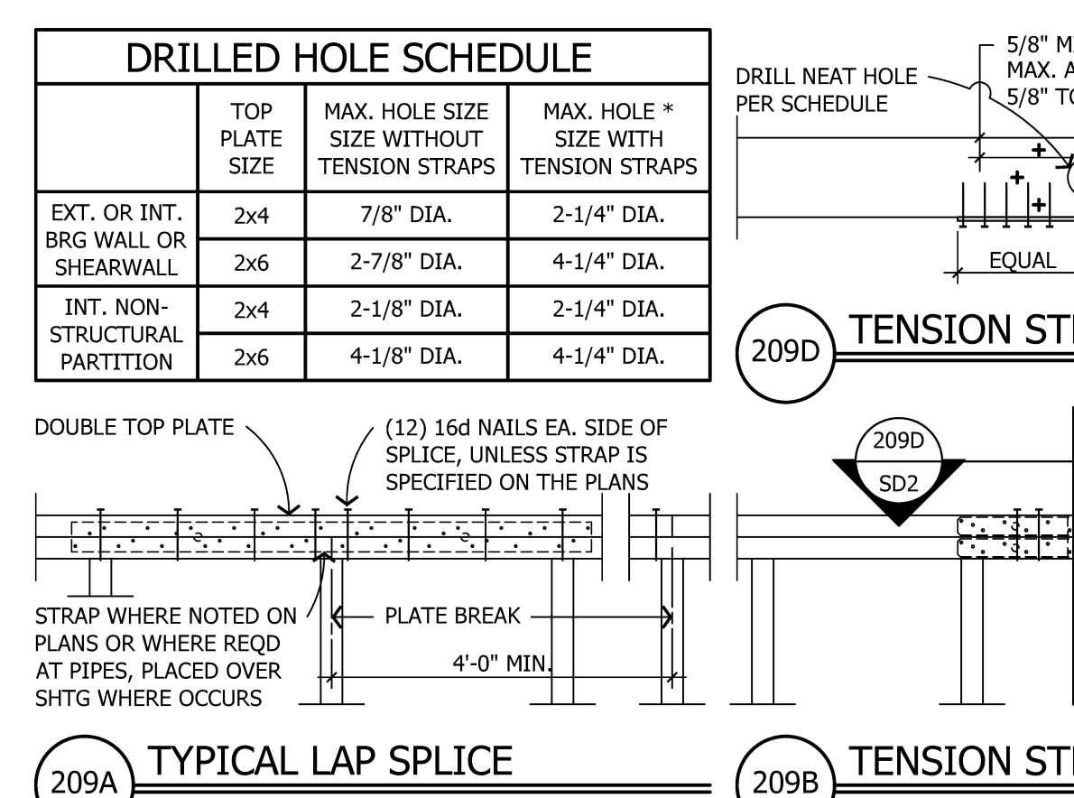
209A TYPICAL LAP SPLICE
