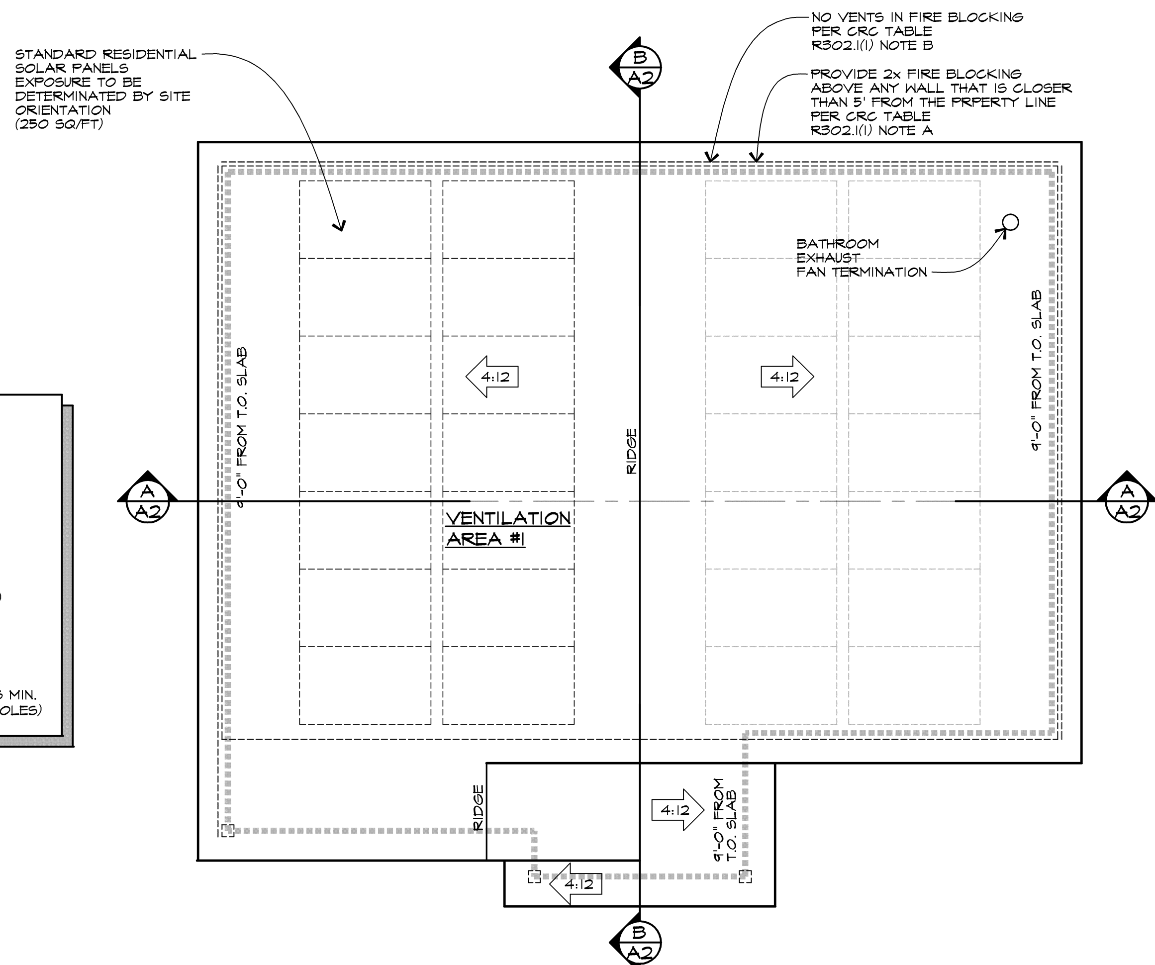
ROOF PLAN
