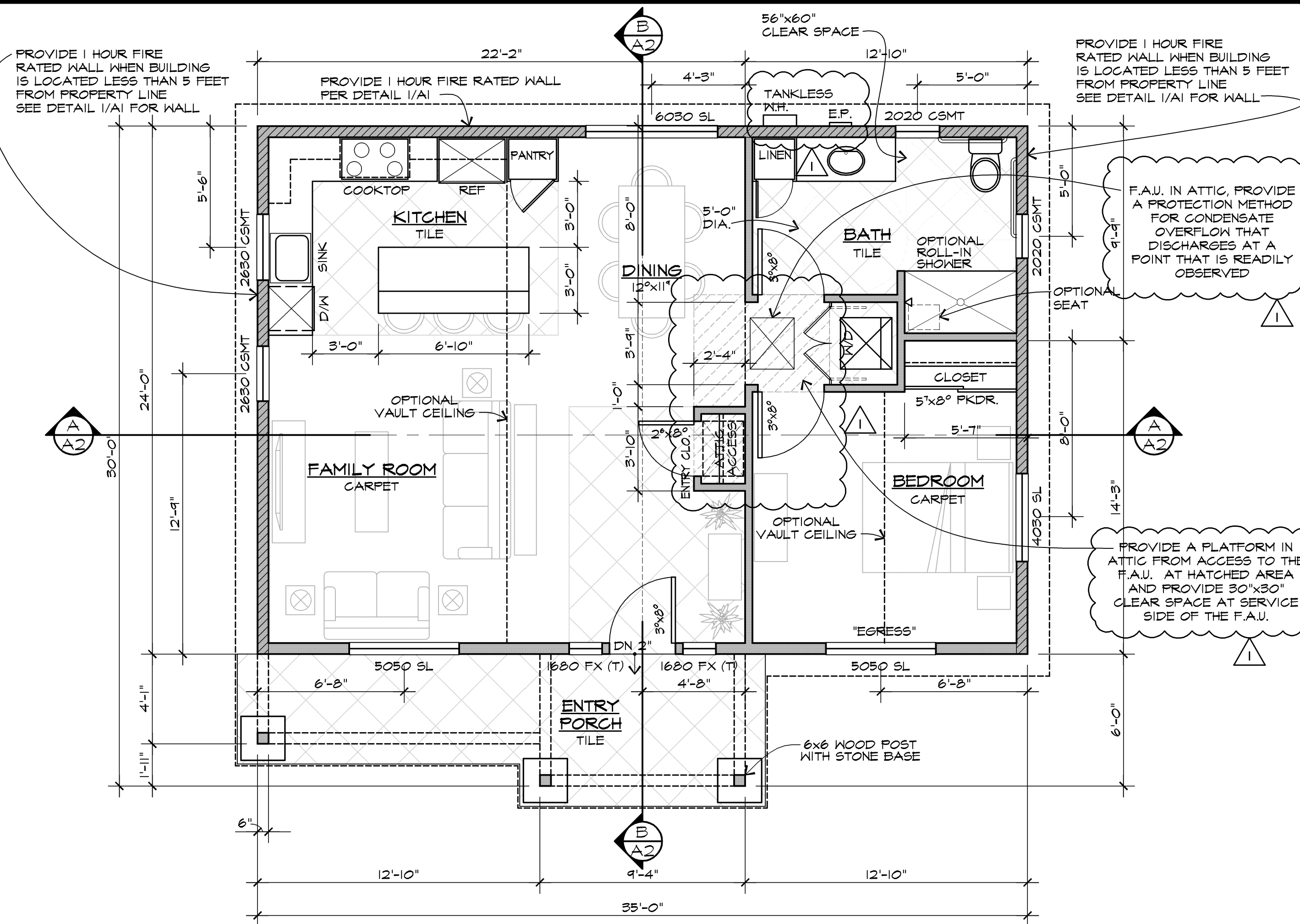
FLOOR PLAN (CRAFTSMAN STYLE)
