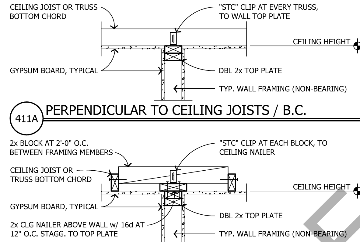
411B PARALLEL TO CEILING JOISTS / B.C.
