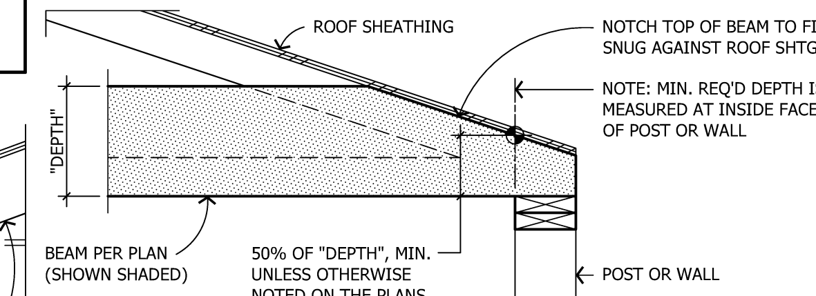
414 SHAPED TOP OF BEAM AT EAVE
