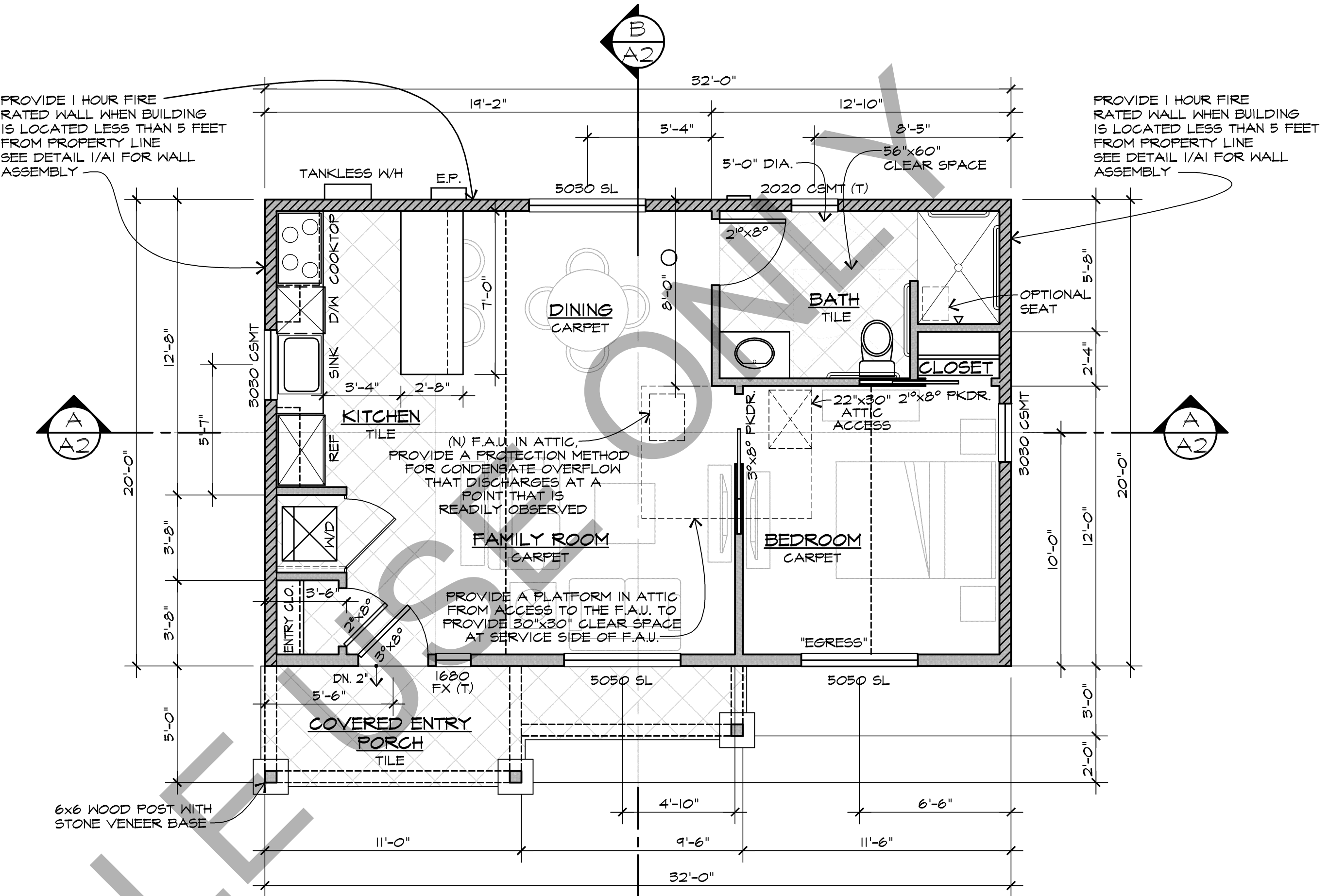
FLOOR PLAN (CRAFTSMAN STYLE)
