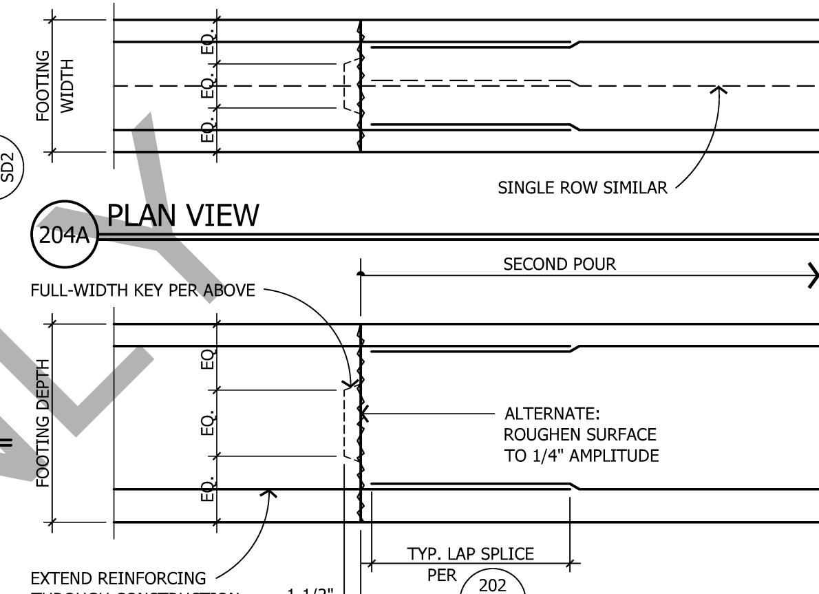
204 FOOTING CONSTRUCTION JOINT
