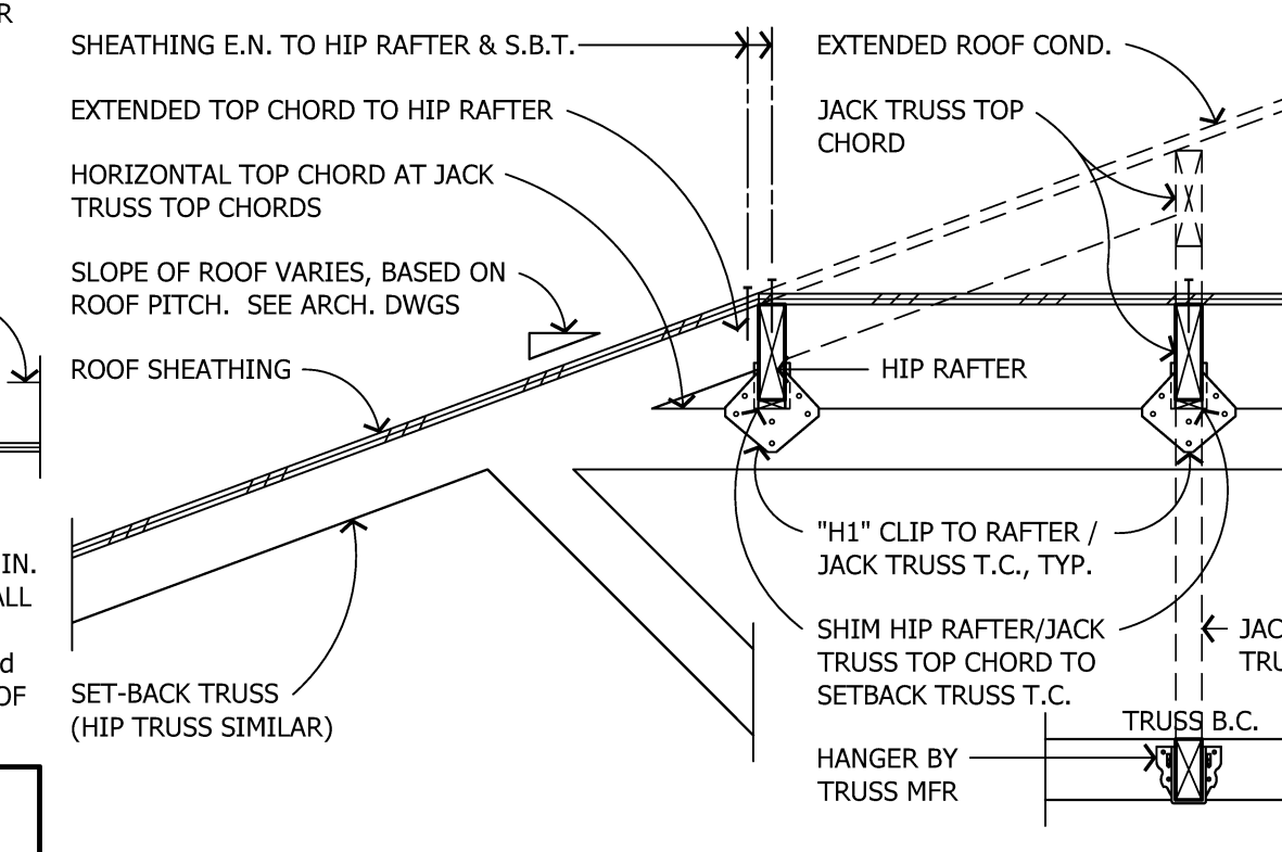
419 CONNECTION AT SET-BACK TRUSS
