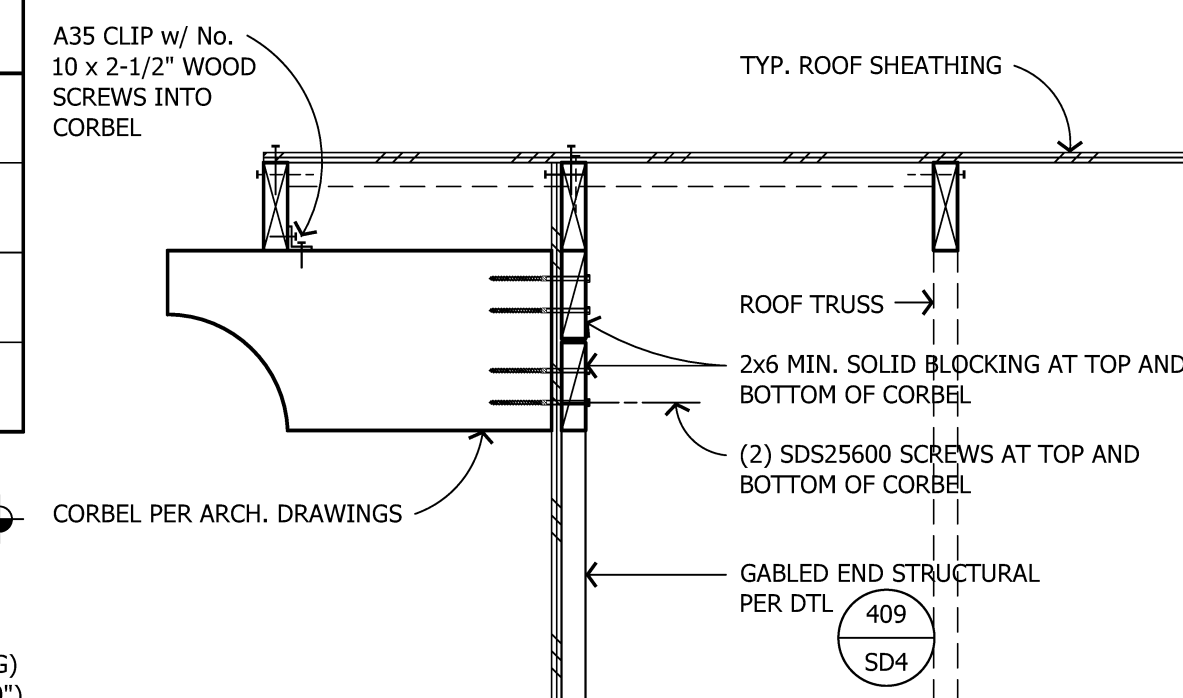
418 CORBEL BEAM AT GABLED END TRUSS
