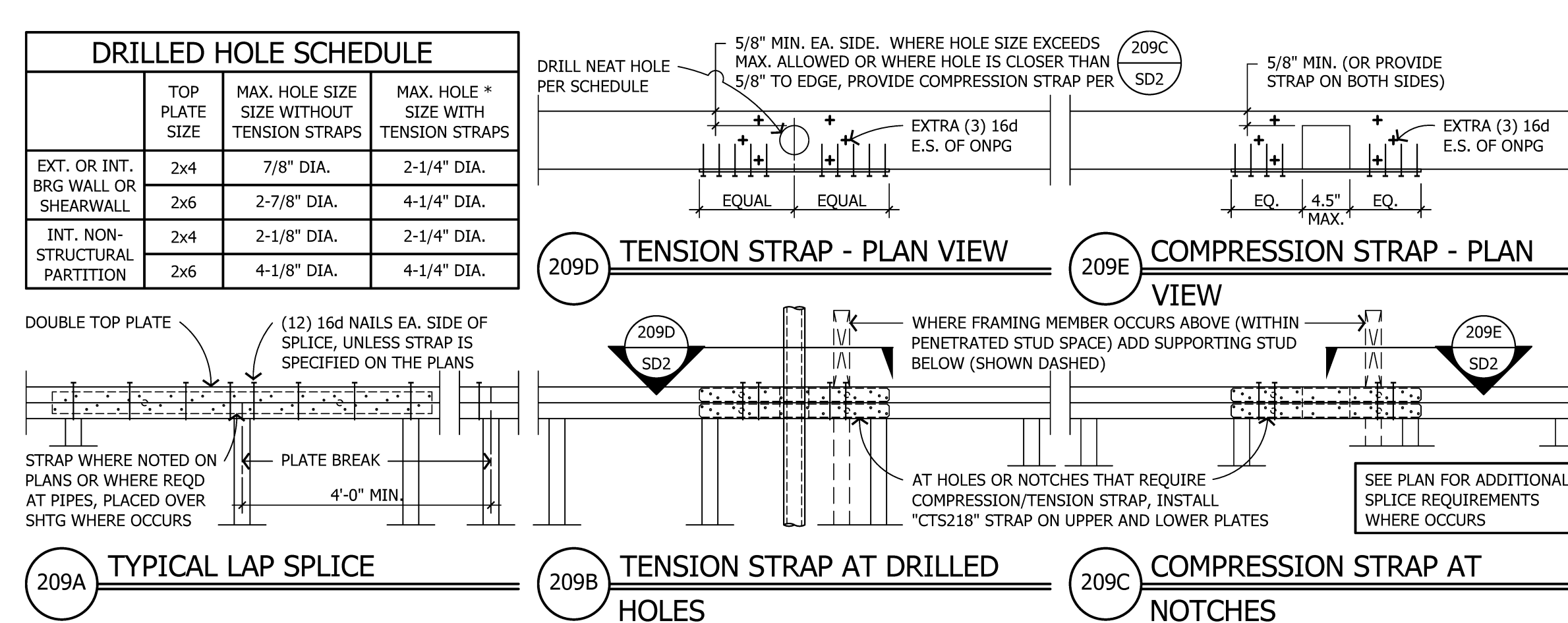
209 TOP PLATE SPLICES, BREAKS AND PENETRATIONS
