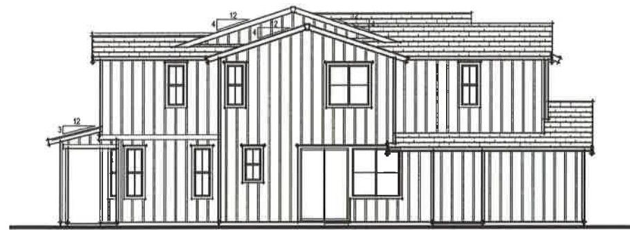
FARMHOUSE 'C' LEFT ELEVATION
