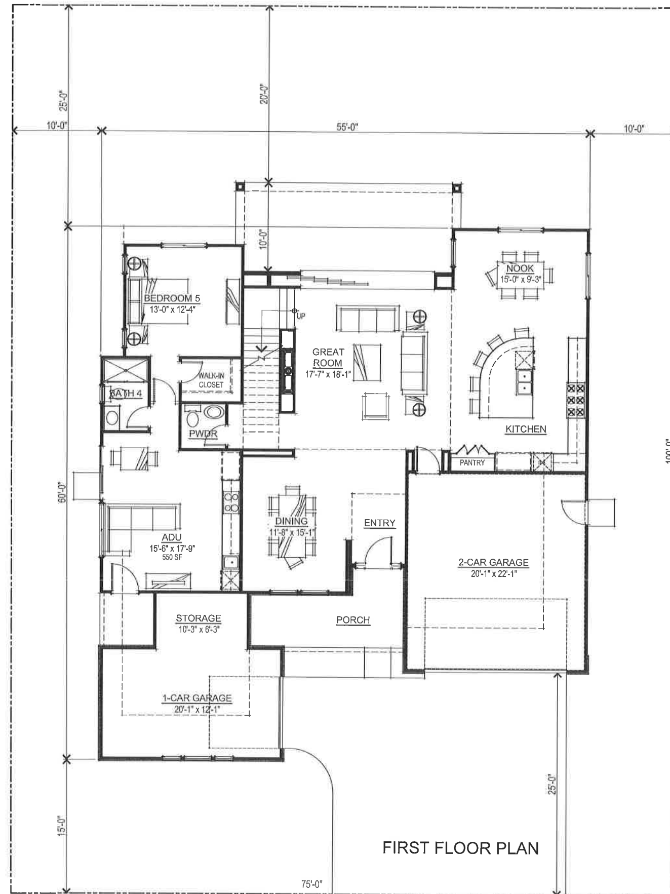
PLAN 2 FLOOR PLANS A006
