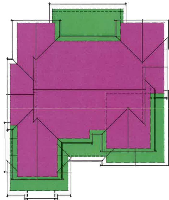
ARTS & CRAFTS 'A' ROOF PLAN
