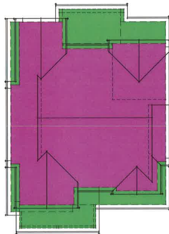
FARMHOUSE 'C' ROOF PLAN
