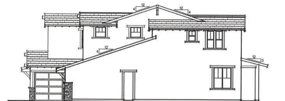
BUNGALOW 'D' RIGHT ELEVATION
