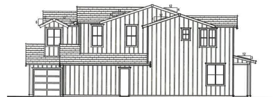
FARMHOUSE 'C' RIGHT ELEVATION
