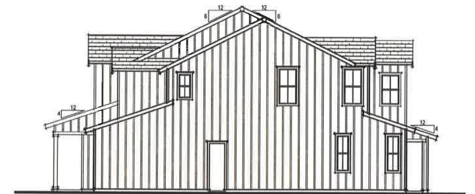
FARMHOUSE 'C' RIGHT ELEVATION
