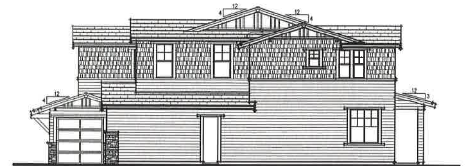
ARTS & CRAFTS 'A' RIGHT ELEVATION
