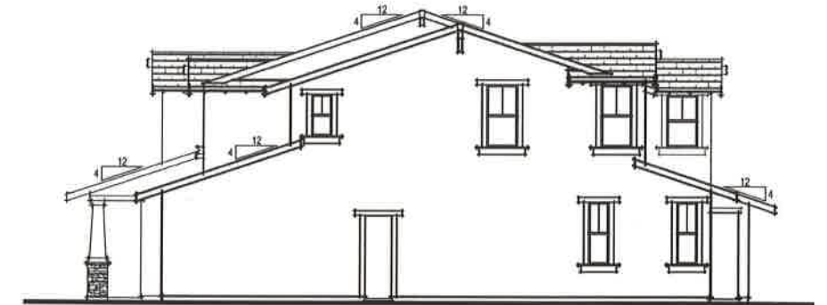
BUNGALOW 'D' RIGHT ELEVATION
