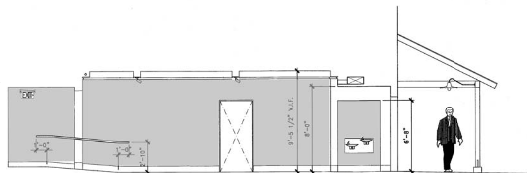
D SOUTH/NORTH - SECTION D 1/4" - 1'-0"
