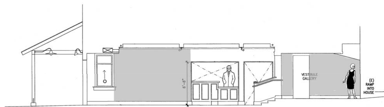
A NORTH/SOUTH - SECTION A 1/4" - 1'-0"
