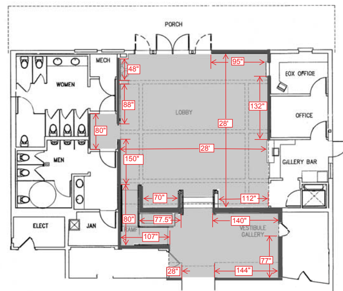
5 KEY PLAN 1/8" - 1'-0"
